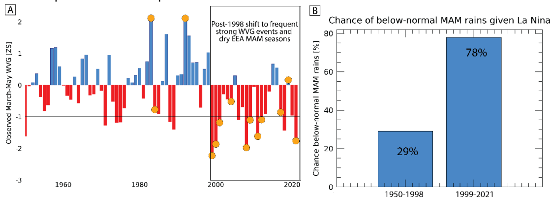
Figure 4. A. Observed March-May Western V Gradient values (bars). Orange circles show below-normal MAM rainy seasons. The time series was standardized using a 1981-2021 baseline. B. Barplot showing frequency of below-normal EEA MAM rains when the prior October-December season was a La Niña event.
